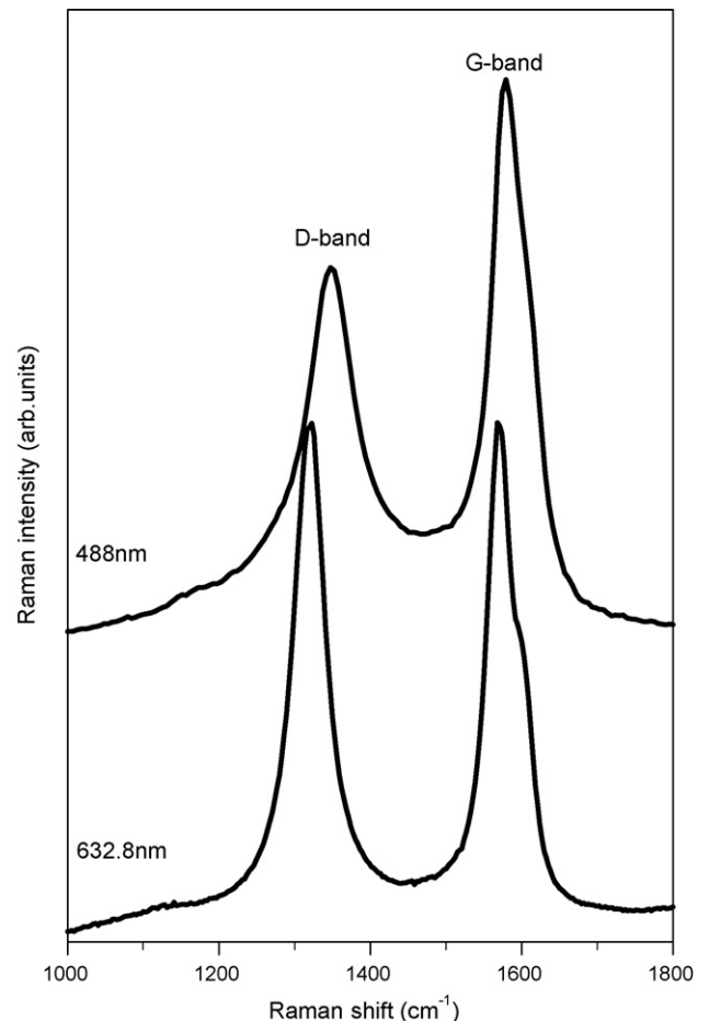
Fig. 3. Micro-Raman spectra of the Sn/C composite film recorded at 488 and 632.8\text{ nm} excitation wavelength.
